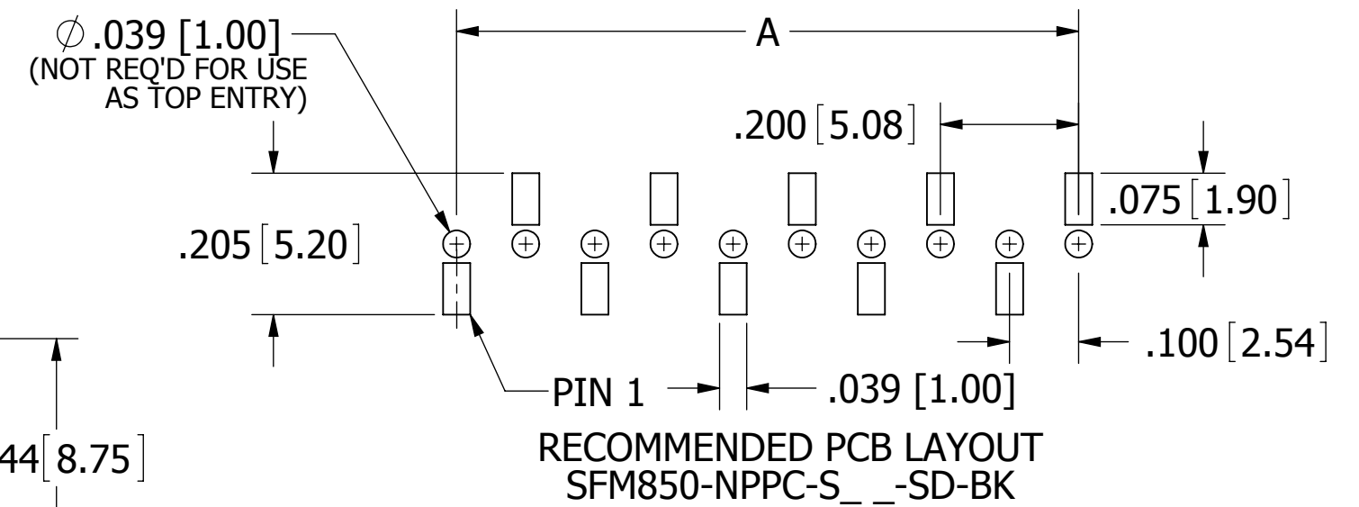
RECOMMENDED PCB LAYOUT SFM850-NPPC-S_-SC-BK
