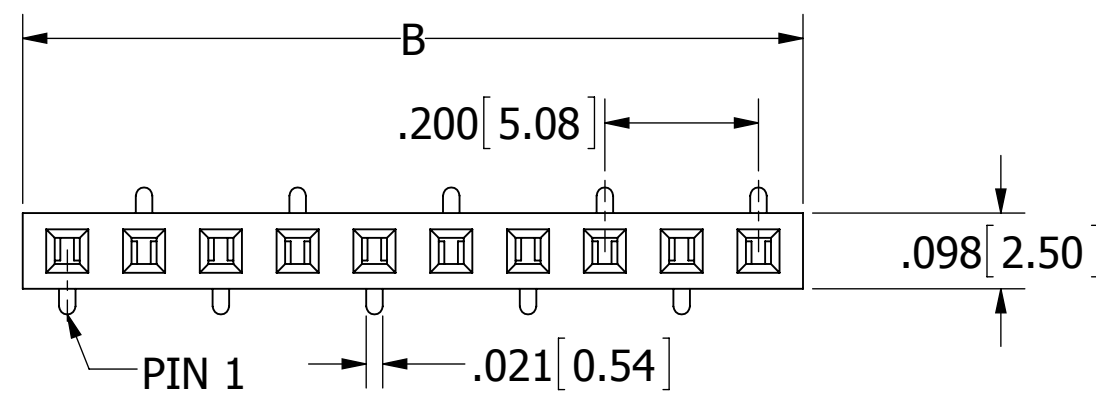
SFM850-NPPC-S_-SD-BK (OPPOSITE BEND, APPLICABLE ON EVEN PIN COUNTS)
