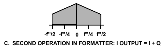
FIGURE 20. QUADRATURE TO REAL CONVERSION OF AN OUTPUT SIGNAL
