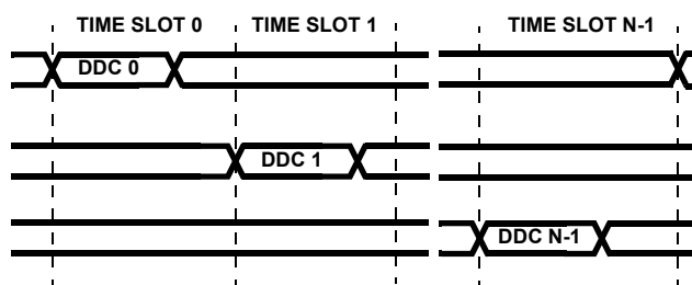
FIGURE 22. TIMING FOR MULTIPLE CHANNEL OPERATION (AUTO THREE-STATE)
