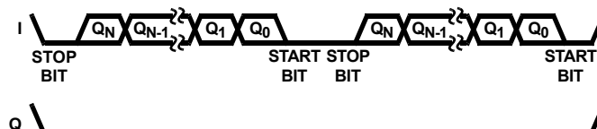
B. I FOLLOWED BY Q OUTPUT MODE FIGURE 10. DATA OUTPUT MODES
