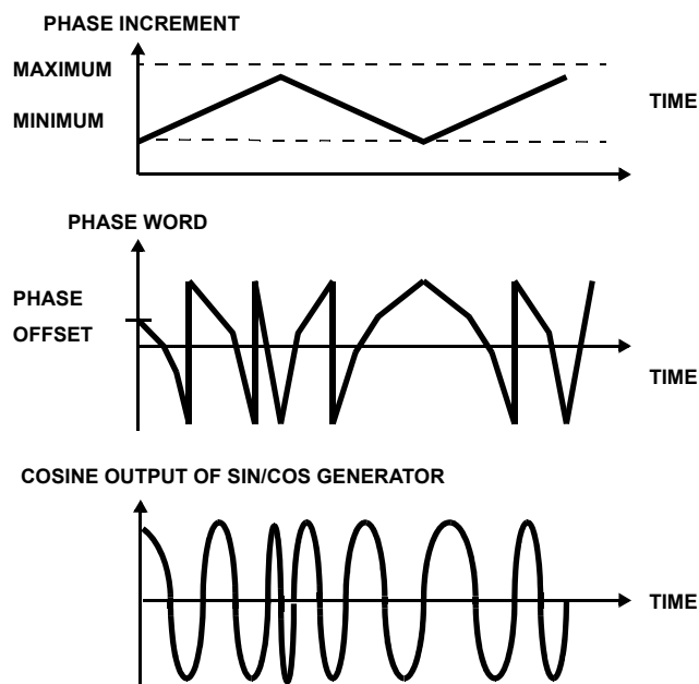
FIGURE 6. UP/DOWN CHIRP
