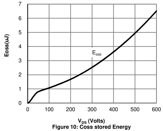
Figure 10: Coss stored Energy
