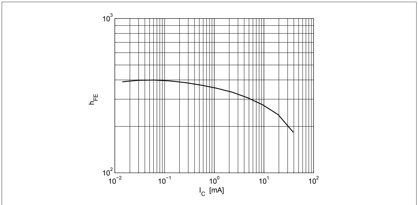
Figure 4 DC current gain h_{FE} = f(I_C) , V_{CE} = 2.5 V
