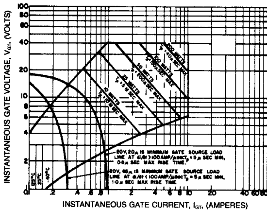
GATE CHARACTERISTICS
