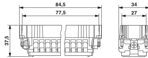
Male insert
