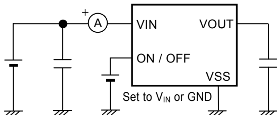
Figure 8 Test Circuit 2
