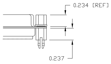
91 ..... 0.237" BOARD SIDE
