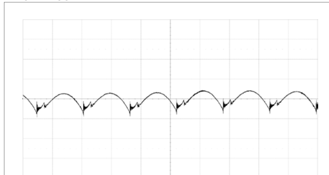
Fundamental output voltage ripple at V_I = 12\text{ V} , I_O = 60\text{ A} , C_{OUT} = 3 \times 470\text{ }\mu\text{F}/4.5\text{ m}\Omega + 10 \times 100\text{ }\mu\text{F} Scale: 5 mV/div, 2 \mu\text{s} /div, 20 MHz bandwidth. See section Output Ripple and Noise.
