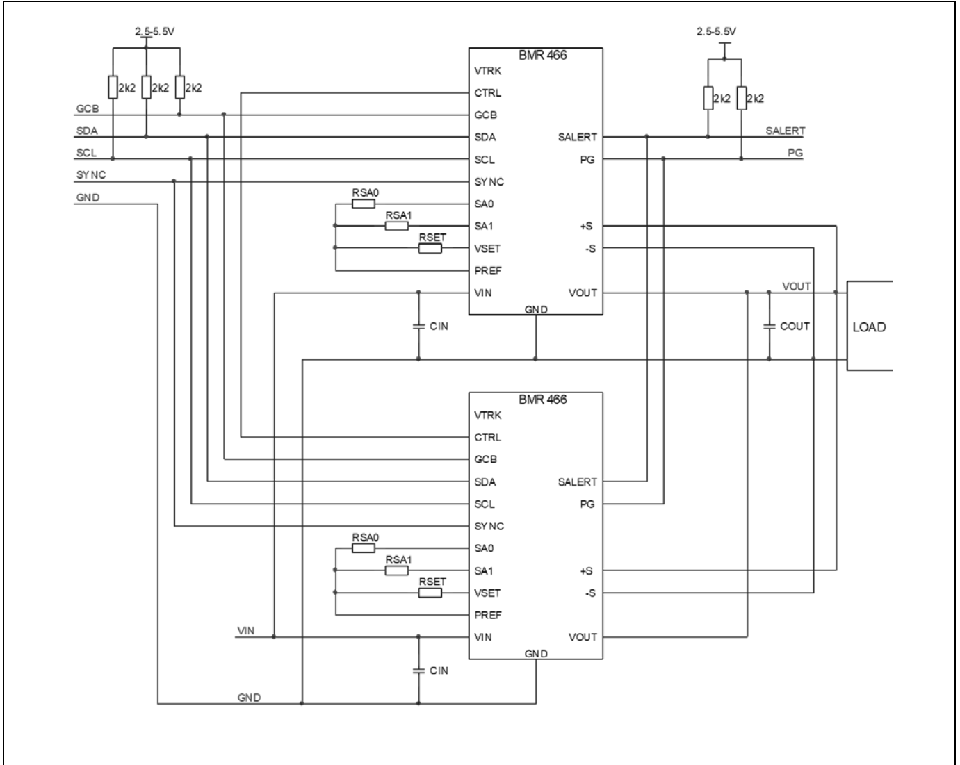
Parallel operation.
