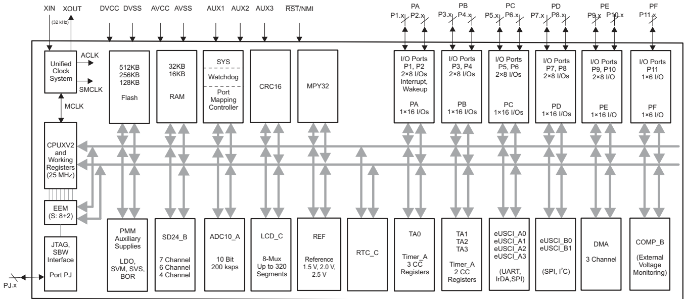
Figure 6-1. Functional Block Diagram – MSP430F677x1PEU, MSP430F676x1PEU, and MSP430F674x1PEU
