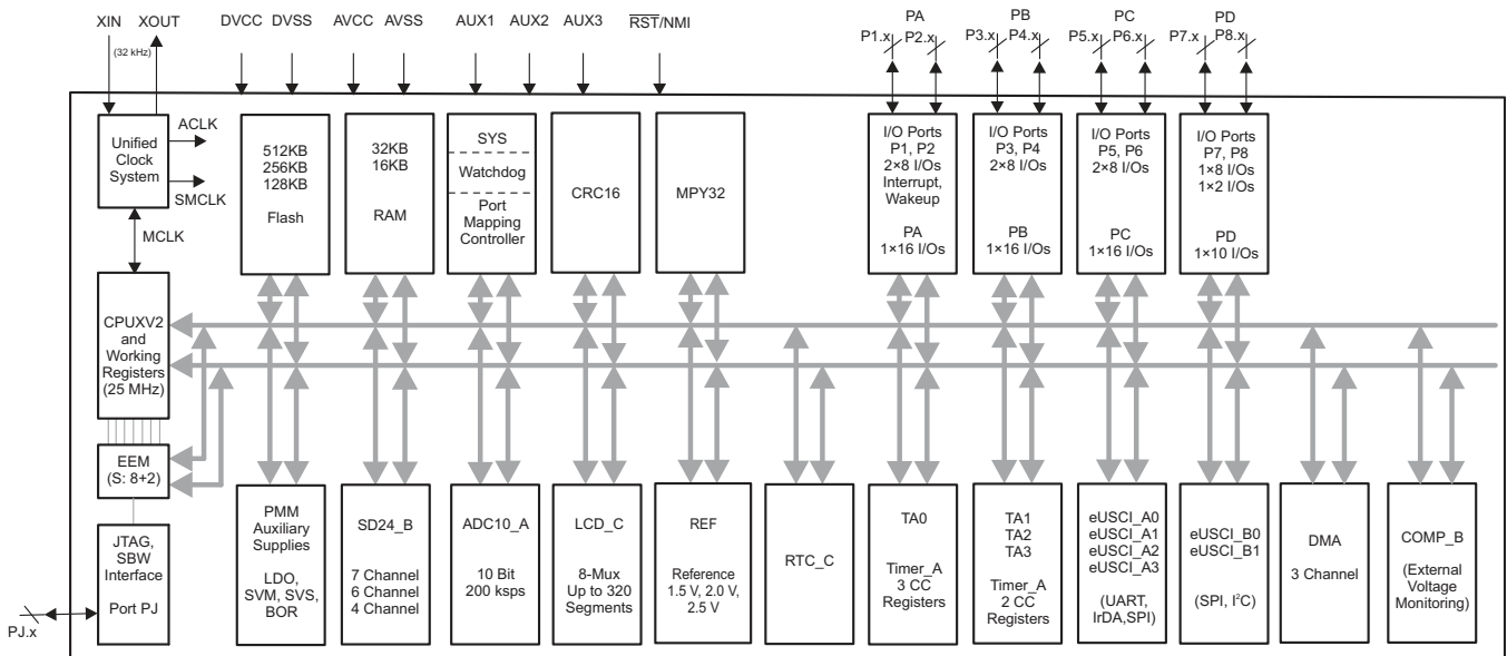
Figure 6-2. Functional Block Diagram – MSP430F677x1PZ, MSP430F676x1PZ, and MSP430F674x1PZ
