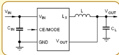
IXD3235 Schematic
