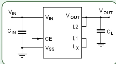
IXD9201/02 Schematic
