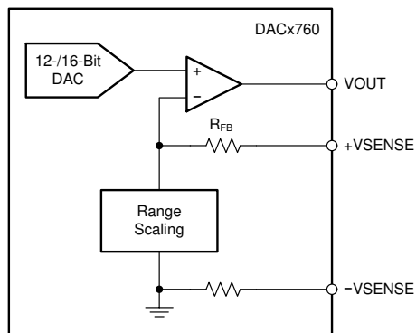
Figure 8-2. Voltage Output
