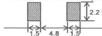
*Recommended Land Pattern (Unit : mm)
