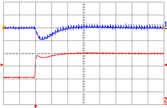
Fig. 1.0V.6: Output voltage response for V_{out} = 1.0\text{ V} to positive load current step change from 10 A to 20 A with slew rate of 5\text{ A}/\mu\text{s} at V_{in} = 12\text{ V} . Top trace: output voltage (200 mV/div.); Bottom trace: load current (5 A/div.). C_o = 100\ \mu\text{F} ceramic. Time scale: 20 \mu\text{s} /div.
