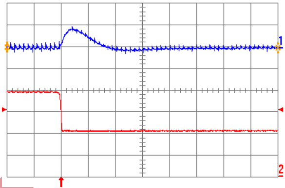
Fig. 1.2V.7: Output voltage response for V_{out} = 1.2\text{ V} to negative load current step change from 20 A to 10 A with slew rate of -5\text{ A}/\mu\text{s} at V_{in} = 12\text{ V} . Top trace: output voltage (200 mV/div.); Bottom trace: load current (5 A/div.). C_o = 100\ \mu\text{F} ceramic. Time scale: 20\ \mu\text{s}/\text{div} .
