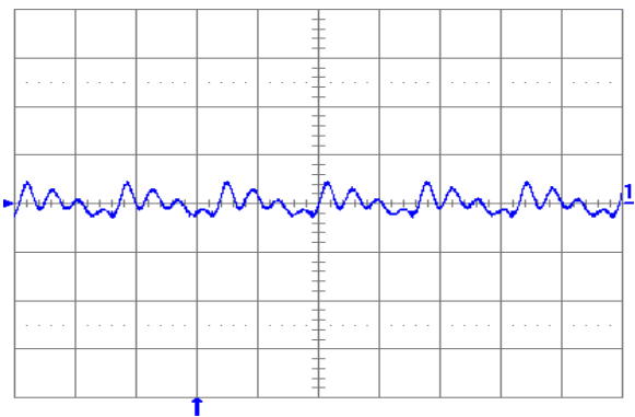
Fig. 1.2V.5: Output voltage ripple (20 mV/div.) at full rated load current into a resistive load with external capacitance 100\text{ }\mu\text{F} ceramic + 1\text{ }\mu\text{F} ceramic and V_{in} = 12\text{ V} for V_{out} = 1.2\text{ V} . Time scale: 2 \mu\text{s} /div.
