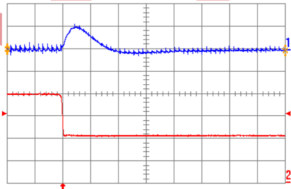
Fig. 1.0V.7: Output voltage response for V_{out} = 1.0\text{ V} to negative load current step change from 20 A to 10 A with slew rate of -5\text{ A}/\mu\text{s} at V_{in} = 12\text{ V} . Top trace: output voltage (200 mV/div.); Bottom trace: load current (5 A/div.). C_o = 100\ \mu\text{F} ceramic. Time scale: 20 \mu\text{s} /div.
