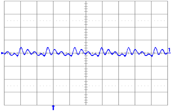
Fig. 1.0V.5: Output voltage ripple (20 mV/div.) at full rated load current into a resistive load with external capacitance 100\ \mu\text{F} ceramic + 1\ \mu\text{F} ceramic and V_{in} = 12\text{ V} for V_{out} = 1.0\text{ V} . Time scale: 2 \mu\text{s} /div.
