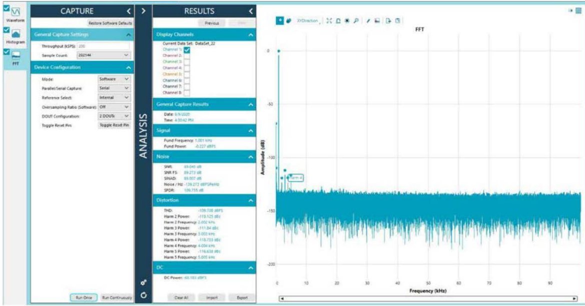
Figure 18. FFT Tab
