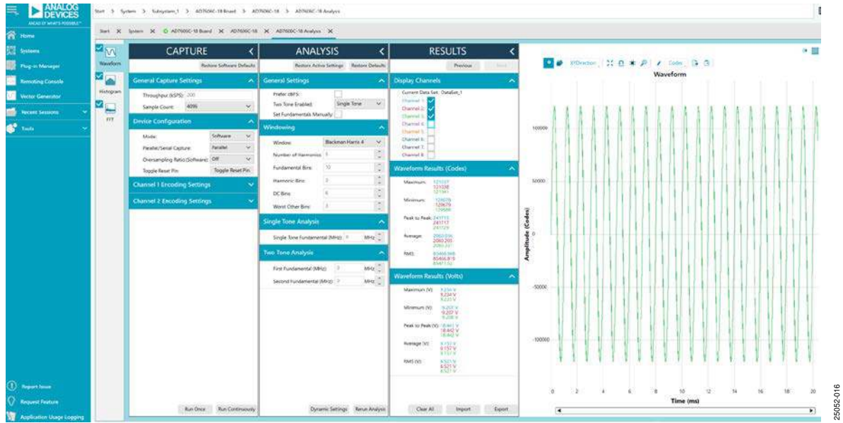
Figure 16. Waveform Tab
