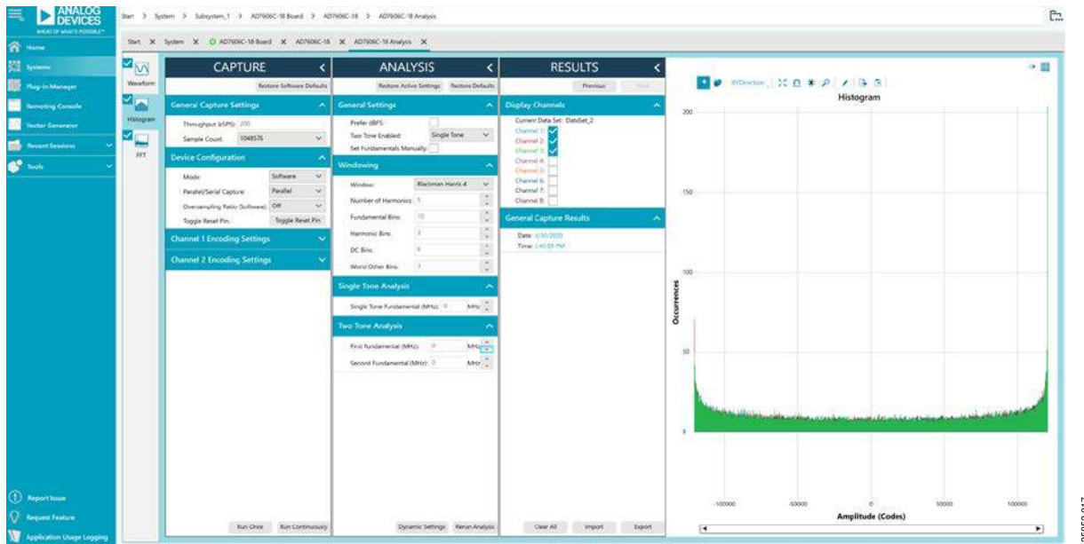
Figure 17. Histogram Tab
