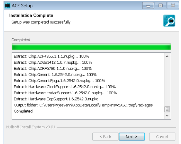
Figure 8. Installation Complete
