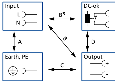
Fig. 19-1: Dielectric strength
