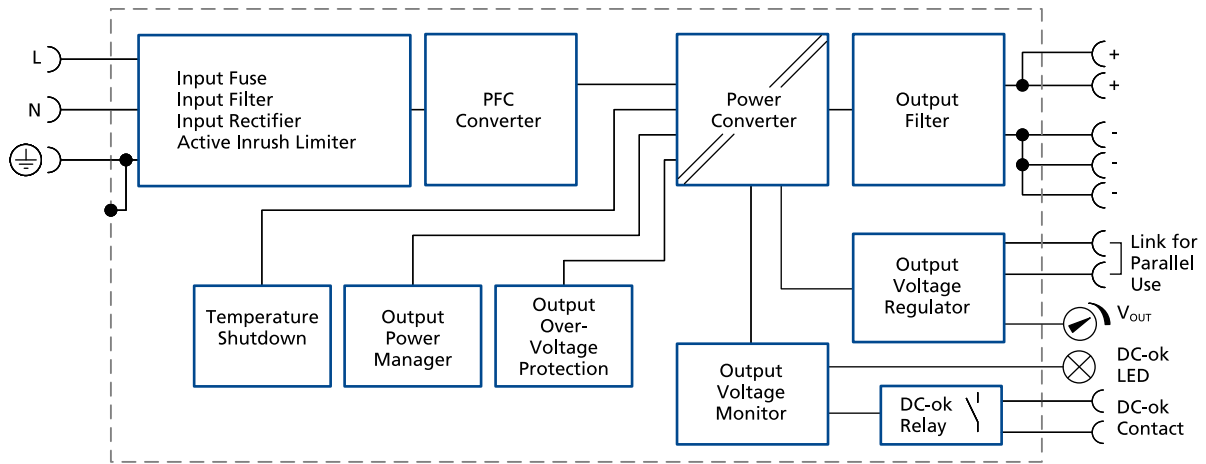
Fig. 12-1: Functional diagram
