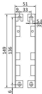
Fig. 23-5: Hole pattern for wall mounting
