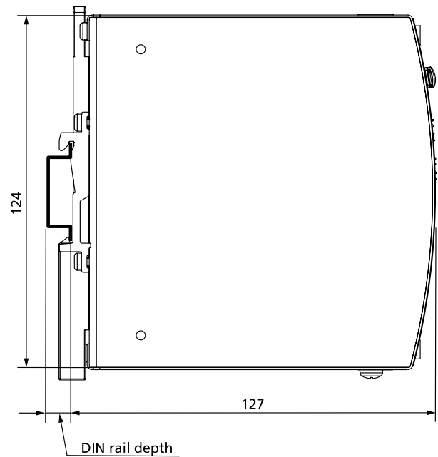
Fig. 22-2: Side view
