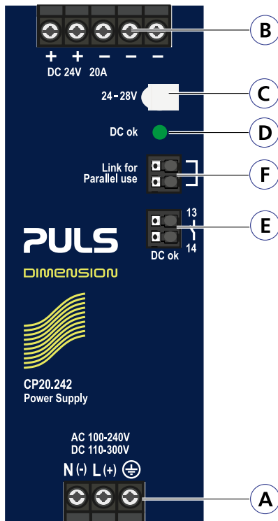
Fig. 14-1: Front side
