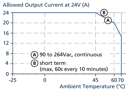
Fig. 16-1: Output current vs. ambient temp. ( I_{nom} = 20A ; I_{out} with PowerBoost = 24A)
