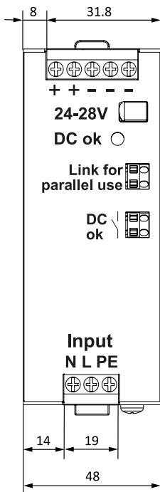
Fig. 22-1: Front view
