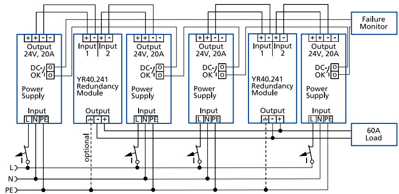
Fig. 24-6: N+1 Redundant configuration for 60A load current with multiple devices and redundancy modules
