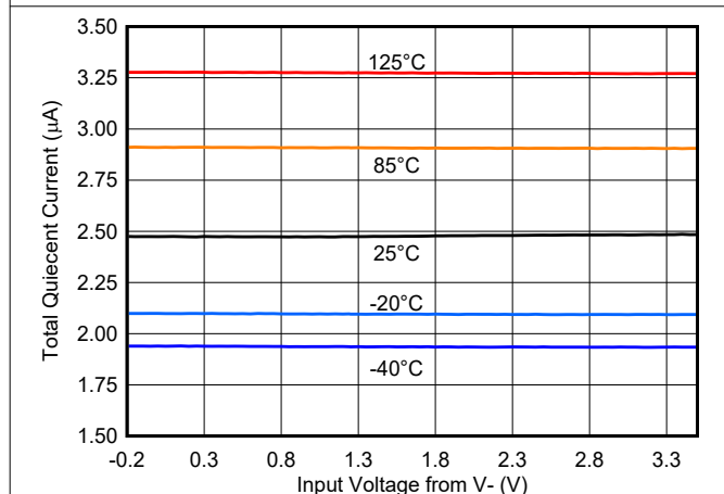
Figure 8-9. Supply Current vs. Common Mode - 3.3V
