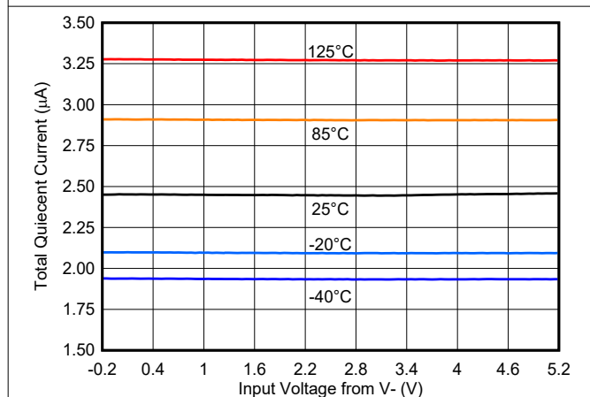
Figure 8-11. Supply Current vs. Common Mode - 5V
