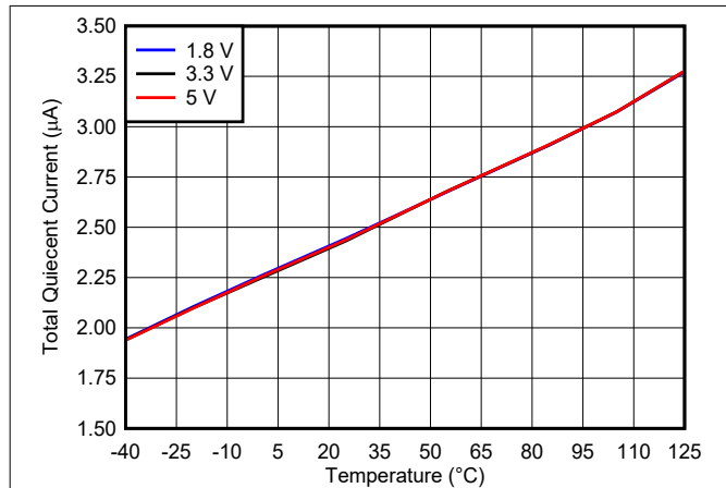
Figure 8-7. Supply Current vs. Temperature
