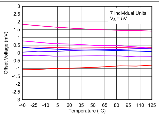
Figure 8-28. Offset Voltage vs. Temperature, 5 V
