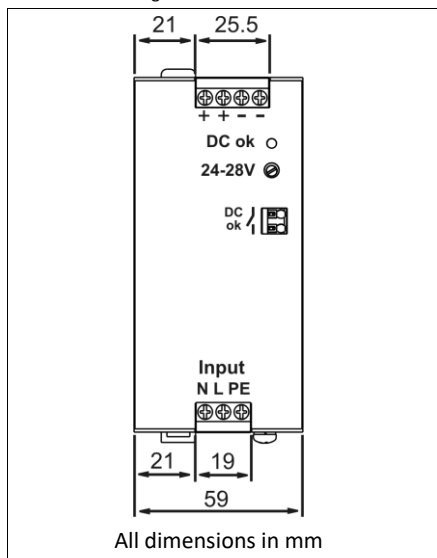
Fig. 21-1 Front view
