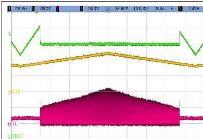
Figure 9-20. 100% Mode Entry and Leave Operation I_{OUT} = 30 mA
