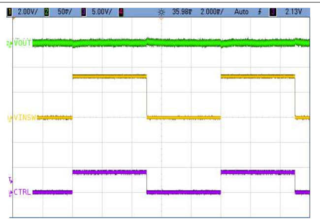
Figure 9-21. VINSW Operation and Control
