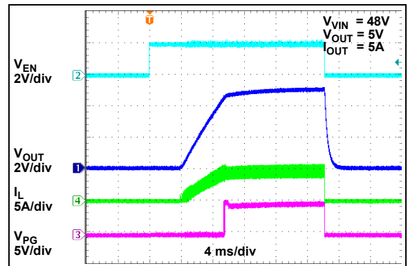
FIGURE 2-35: Enable Turn-On/Turn-Off.
