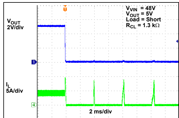
FIGURE 2-48: Output Short Circuit.
