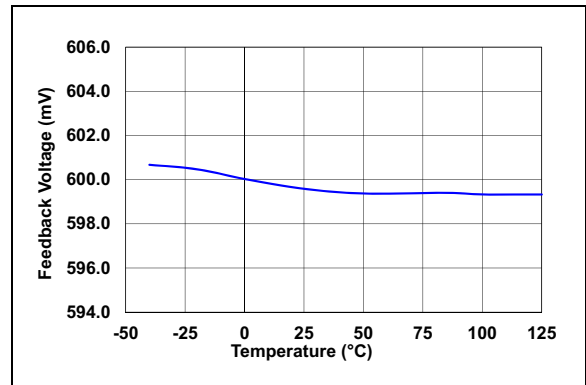
FIGURE 2-18: Feedback Voltage vs. Temperature.
