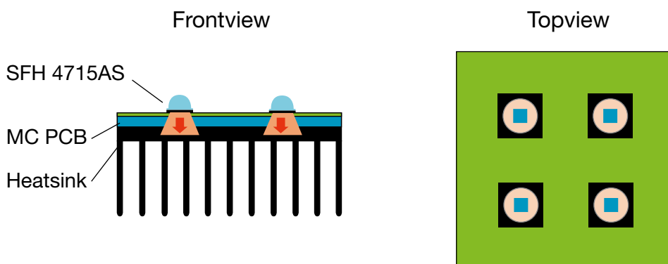
Figure 6: Design example
