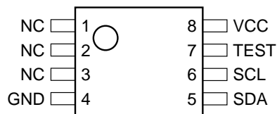
8-Pin TSSOP
