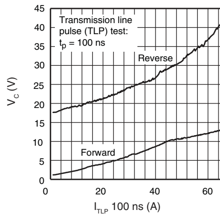
Fig. 9 - Typical Peak Clamping Voltage vs. TLP current (TLP = transmission line pulse; t_p = 100 ns)
