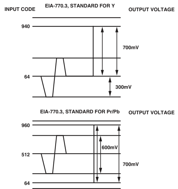
Figure 94. EIA 770.3 Standard Output Signals (1080i, 720p)
