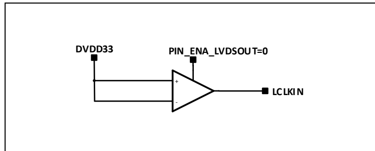
Figure 44: LCLKIN Input
