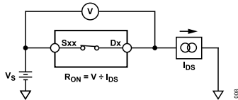
Figure 22. On Resistance
