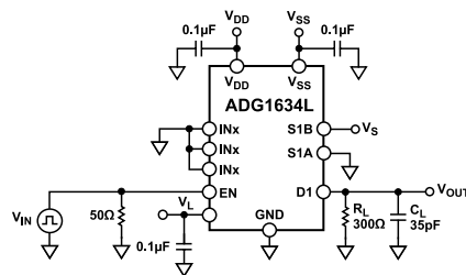
Figure 27. Enable Delay On Time, t_{\text{ON}}(\text{EN}) and Enable Delay Off Time, t_{\text{OFF}}(\text{EN})
