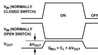
Figure 28. Charge Injection
