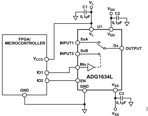
Figure 33. Typical Application
