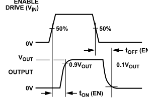
Figure 27. Enable Delay On Time, t_{\text{ON}}(\text{EN}) and Enable Delay Off Time, t_{\text{OFF}}(\text{EN})
