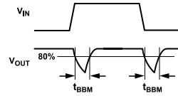
Figure 26. Break-Before-Make Delay, t_{\text{BBM}}
