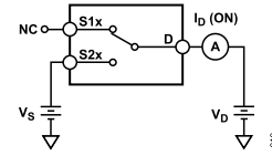
Figure 24. On Leakage
