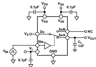
Figure 28. Charge Injection
