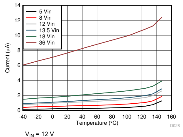
Figure 7-6. Shutdown Current
