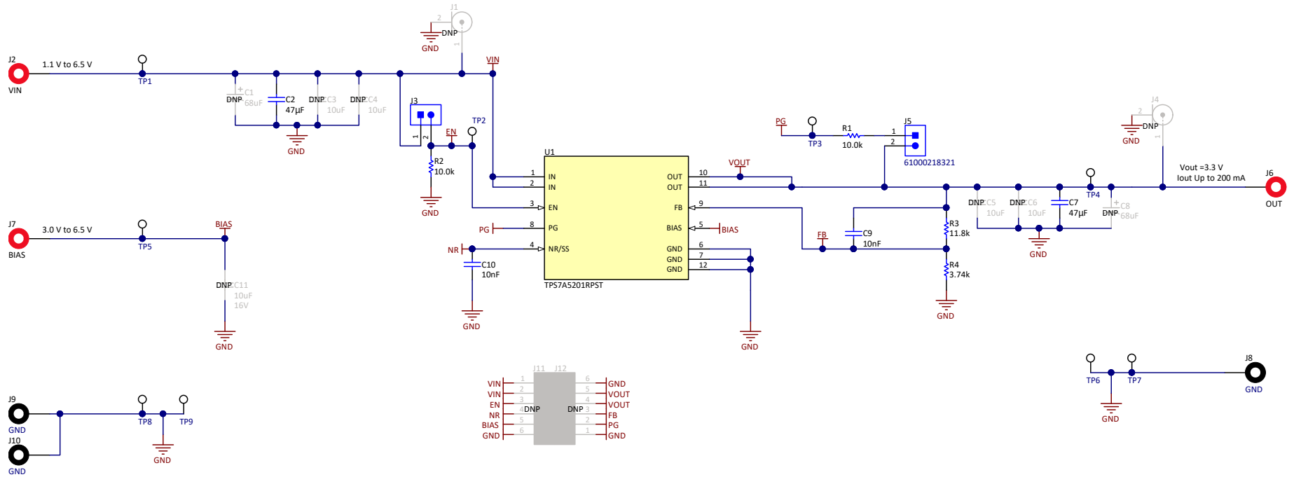
Figure 6. TPS7A52EVM-031 Schematic
