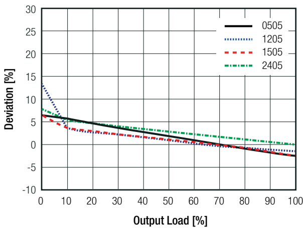
RI3-xx05S
