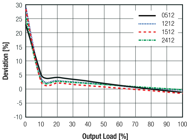
RI3-xx12S
