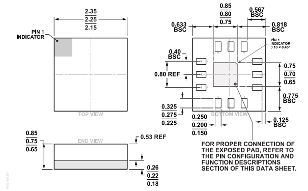
Figure 26. 12-Terminal Land Grid Array [LGA] 2.25 mm x 2.25 mm Body and 0.75 mm Package Height (CC-12-3) Dimensions shown in millimeters
