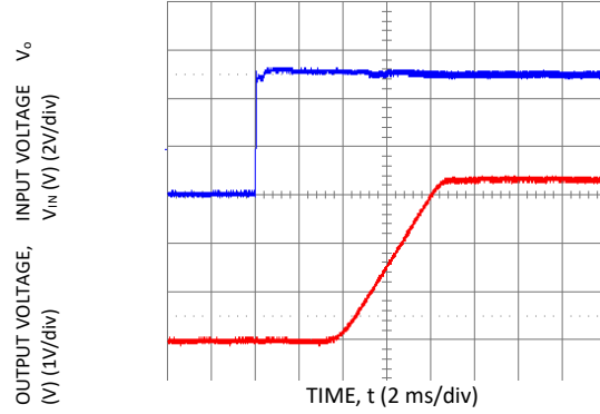
Figure 16. Typical Start-Up with application of V_{in} with ( V_{in} = 5.0 Vdc, V_o = 3.3 Vdc, I_o = 5 A).
