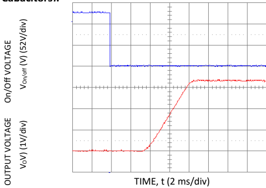
Figure 14. Typical Start-Up Using Remote On/Off ( V_{in} = 5 Vdc, V_o = 3.3 Vdc, I_o = 5.0 A).
