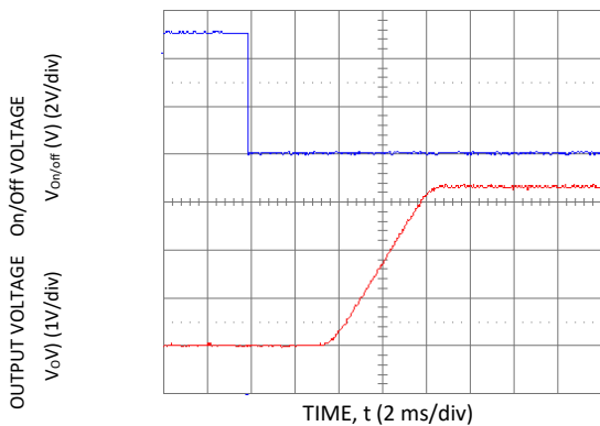
Figure 15. Typical Start-Up Using Remote On/Off with Low-ESR external capacitors (7x150uF Polymer) ( V_{in} = 5 Vdc, V_o = 3.3 Vdc, I_o = 5.0 A, C_o = 1050 \mu F).
