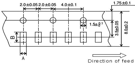
<Paper Tape W8P2>
