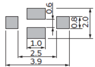
(in mm) NFM3DCC/3DPC
