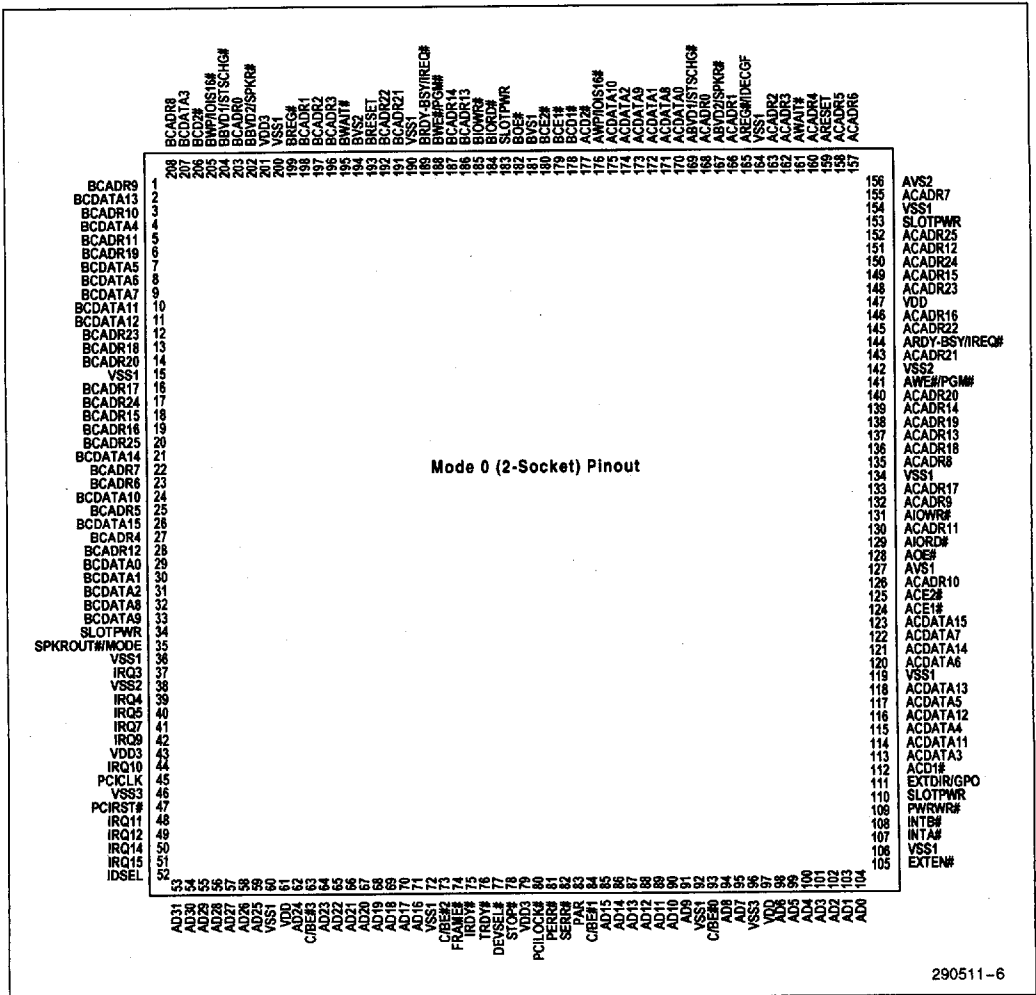
Figure 4. Mode 0 Pinout
