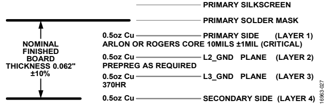
Figure 27. 4-Layer Stackup
