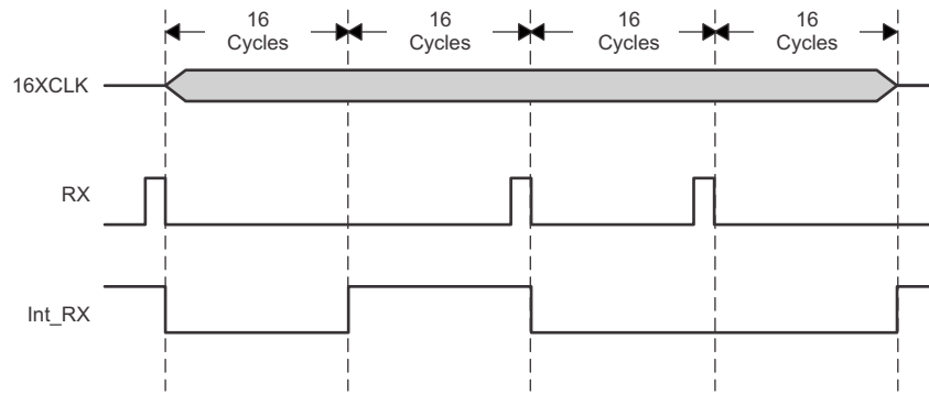
Figure 42. Positive RX Pulse Decode – Macro View
