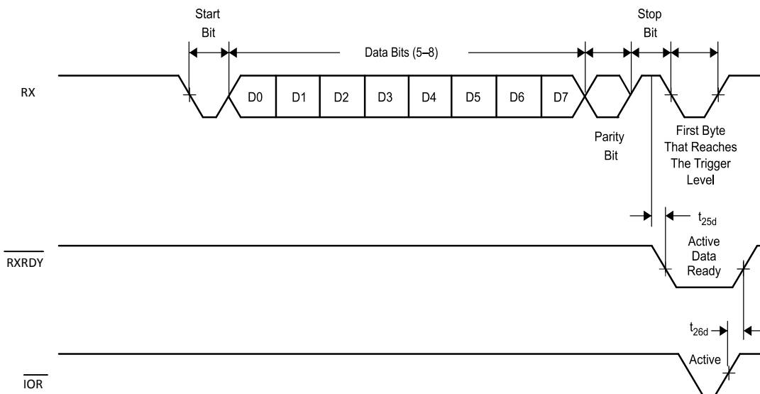
Figure 12. Receive Timing in FIFO Mode ( \overline{IOR} and \overline{IOW} Mode, MODE = VCC)
