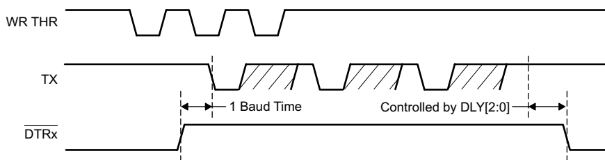
Figure 31. DTRx and Transmit Data Relationship
