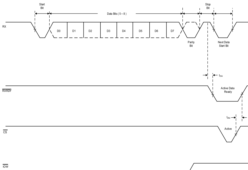
Figure 11. Receive Ready Timing in Non-FIFO Mode ( \overline{IOW} Only Mode, MODE = GND)
