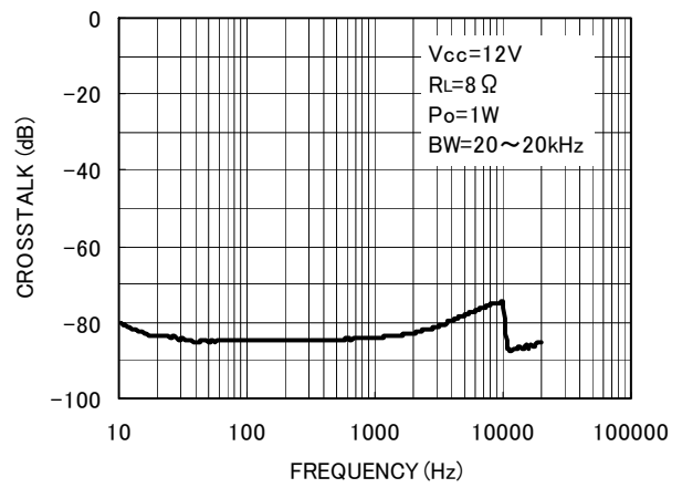
Fig. 4 Crosstalk - Frequency
