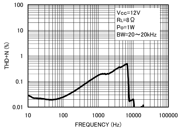
Fig. 2 THD+N – Frequency
