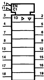
CD74FCT373, CD74FCT373AT TYPES
