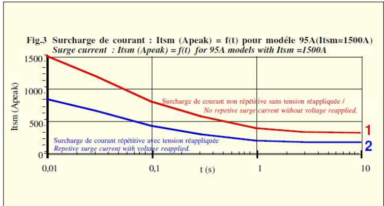
Fig.3 Surcharge de courant : Istm (Apeak) = f(t) pour modèle 95A (Istm=1500A) Surge current : Istm (Apeak) = f(t) for 95A models with Istm =1500A 1 - No repetitive Istm is given without voltage reappplied. This curve is used to define the protection (fuses). 2 - Repetitive Istm is given for inrush current with initial Tj = 70°C. In normal operation, this curve mustn't be exceeded. Be careful, the repetition of the surge current decreases the life expectancy of the SSR.
