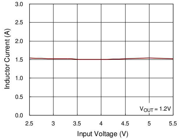
Inductor Current Limit vs. Input Voltage
