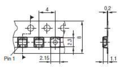
Figure 1 Outline PG-SOT323, dimensions in mm
