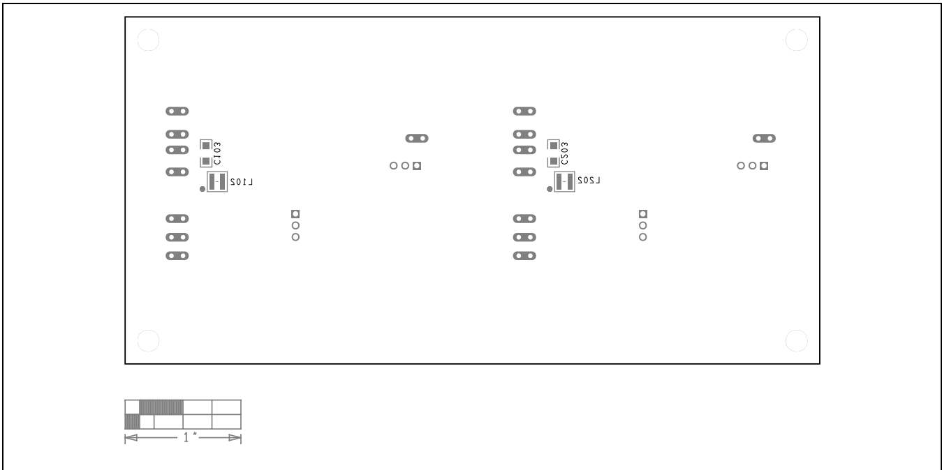
MAX17573 EV Kit Component Placement Guide—Bottom Silkscreen
