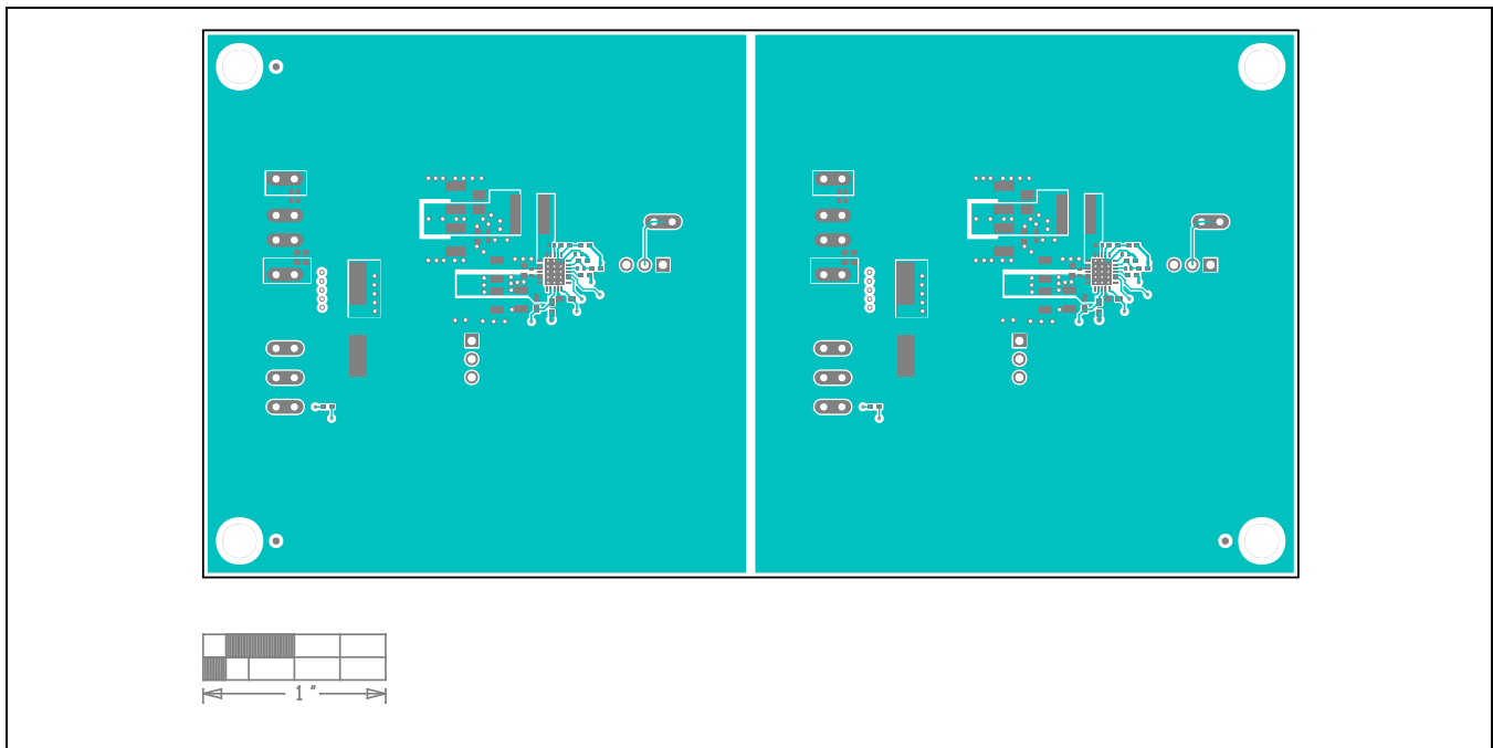
MAX17573 EV Kit PCB Layout—Top
