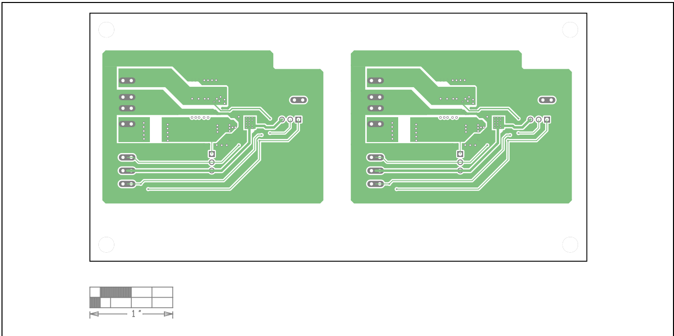
MAX17573 EV Kit PCB Layout—Layer 3
