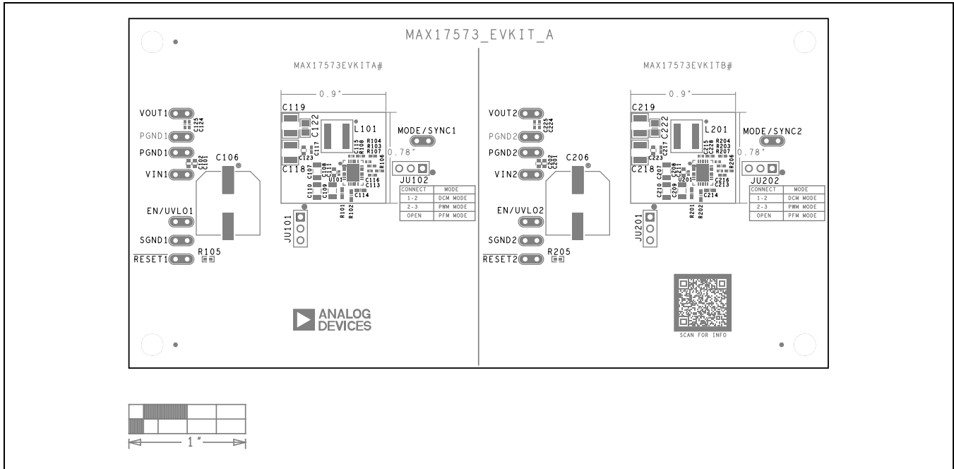
MAX17573 EV Kit Component Placement Guide—Top Silkscreen
