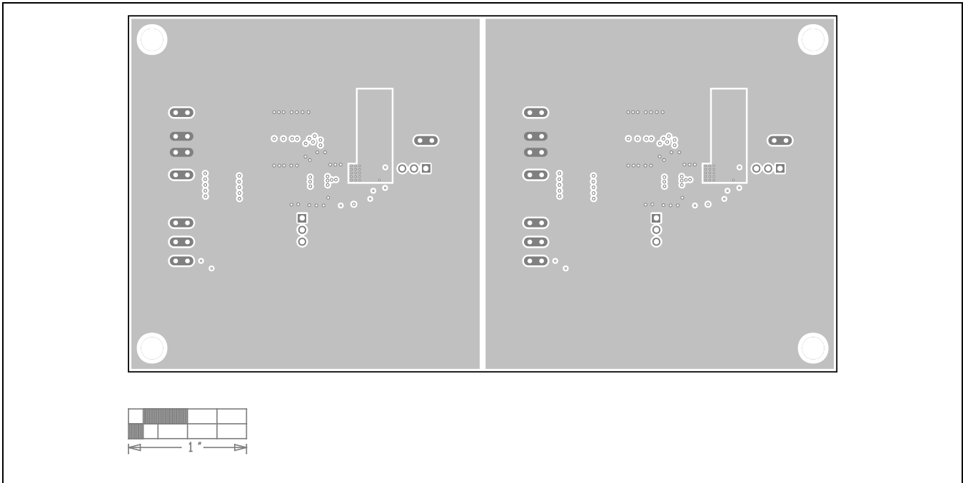
MAX17573 EV Kit PCB Layout—Layer 2
