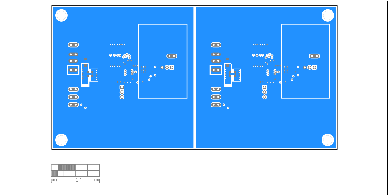
MAX17573 EV Kit PCB Layout—Bottom
