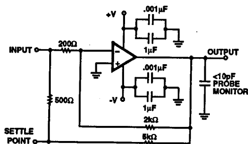
FIGURE 4. SETTLING TIME CIRCUIT
