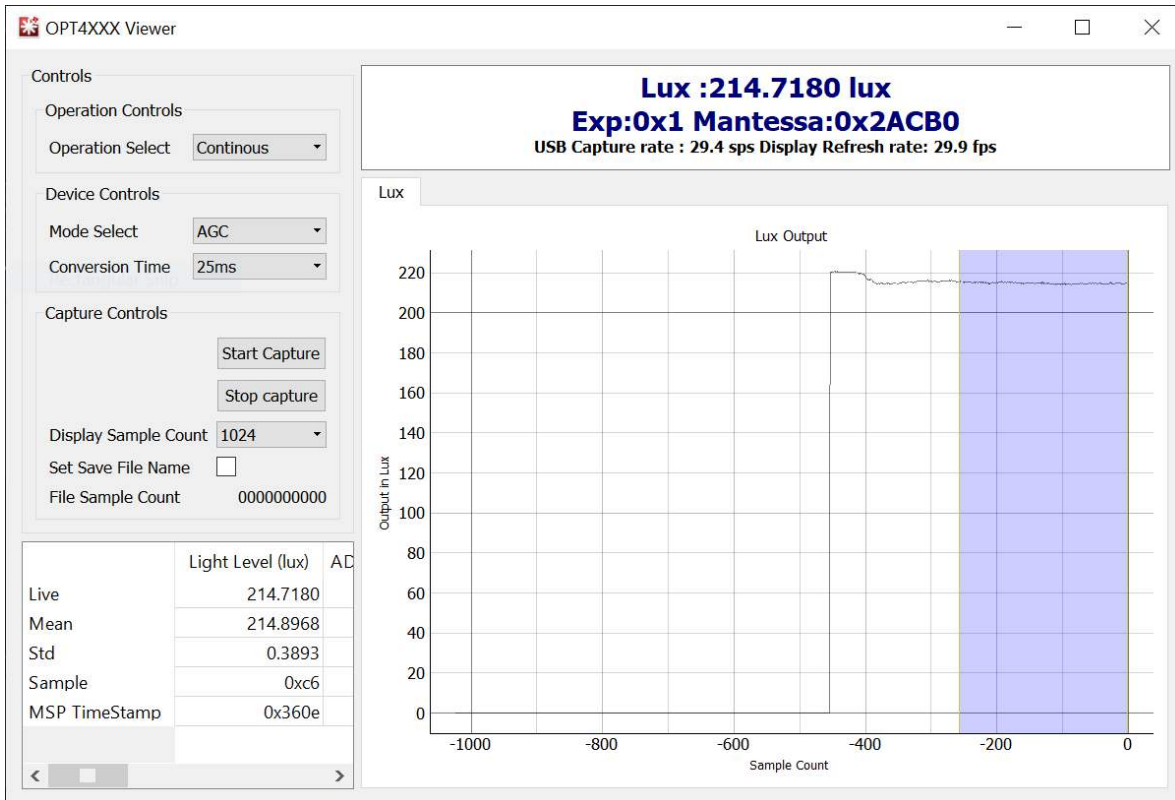
Figure 3-13. GUI Capture Running
