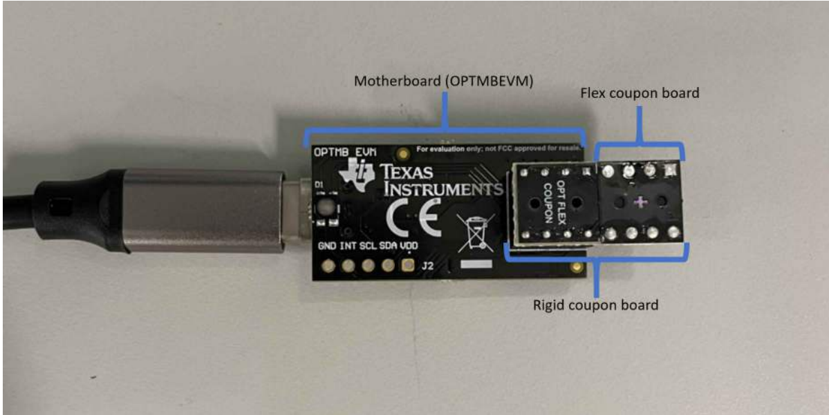
Figure 4-1. OPT4001YMNEVM construction
