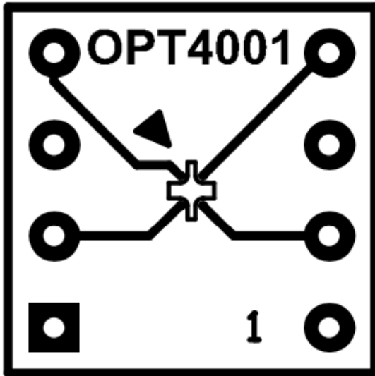
Figure 4-3. PCB Top Layer
