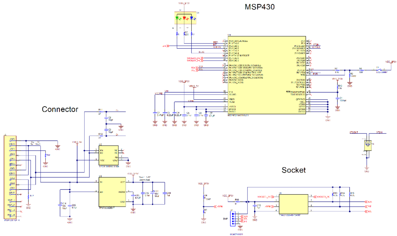
Figure 4-12. OPTMBEVM Schematic
