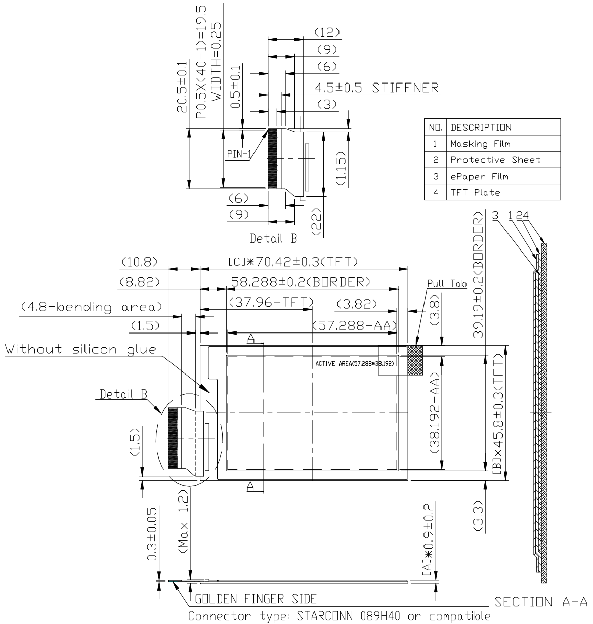
Figure 1-1 EPD Drawing
