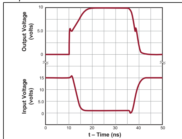
FIGURE 2-6: Switching Waveform.
