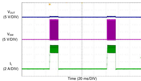
Figure 9-20. LM62435-Q1 Short Circuit Protection
