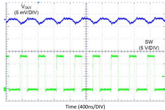
Figure 9-18. LM62435-Q1 Switching Waveform and V_{OUT} Ripple
