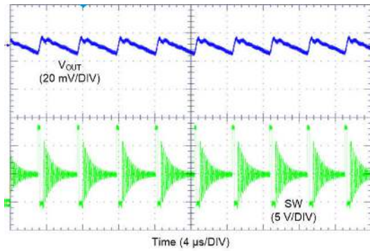
Figure 9-17. LM62435-Q1 Switching Waveform and V_{OUT} Ripple
