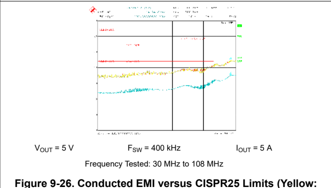
Figure 9-26. Conducted EMI versus CISPR25 Limits (Yellow: Peak Signal, Blue: Average Signal)
