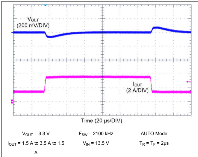
Figure 9-23. LM62435-Q1 Load Transient
