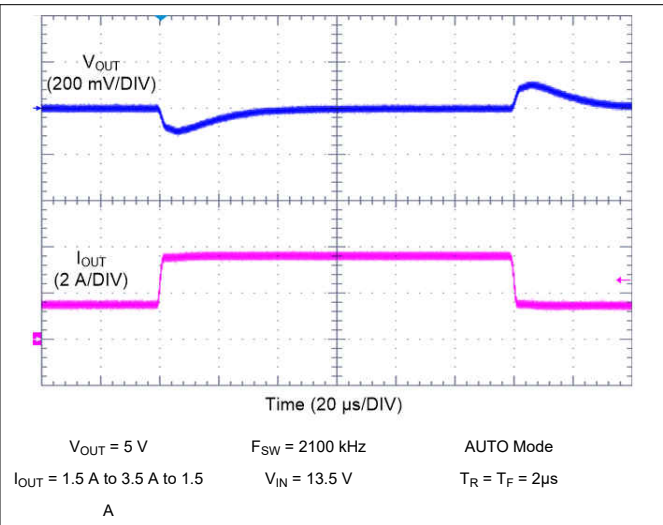
Figure 9-24. LM62435-Q1 Load Transient
