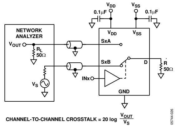
Figure 19. Channel-to-Channel Crosstalk
