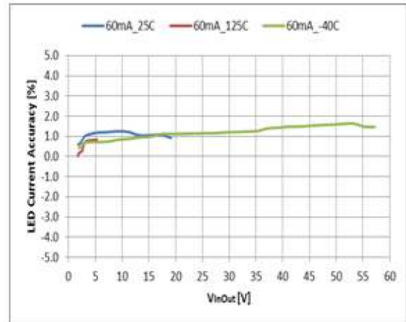
Figure 10 LED Current Accuracy (%) vs. VinOut across Temp
