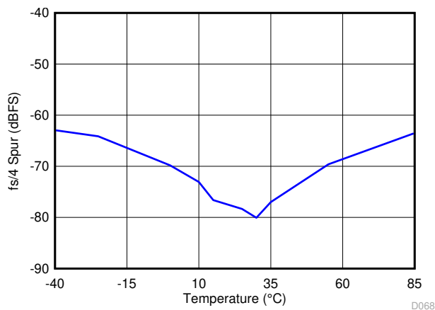
Figure 9-5. Variation of the f_S / 4 Spur Over Temperature
