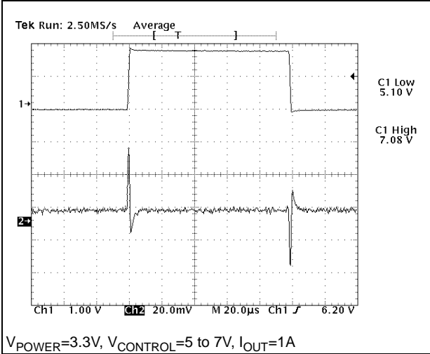
Figure 14. Line transient response V_{Power}=3.3\text{ V}
