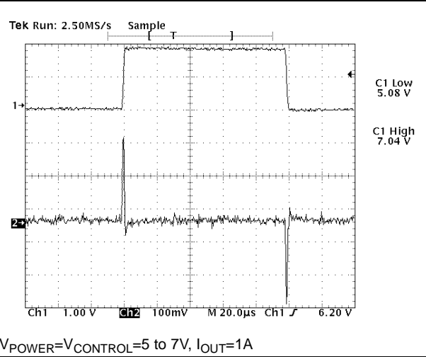
Figure 15. Line transient response V_{Power}=5\text{ V}
